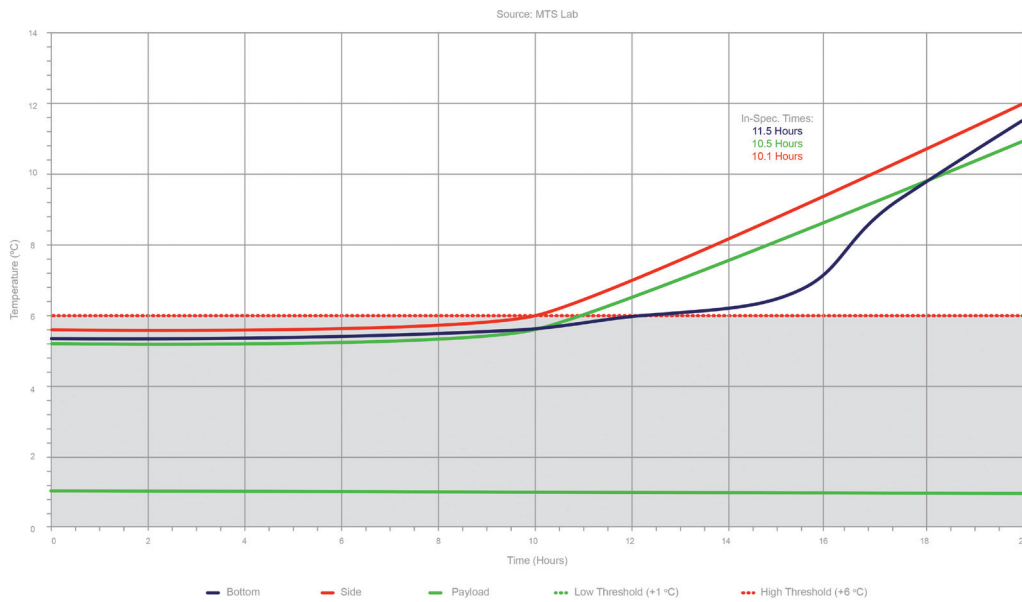
GH02 Operating Room Container Thermal Validation Test Results (Cool +20 Deg. C Ambient; 3 Water Payload Bags; 24 hours in the Refrigerator After Freezing)
